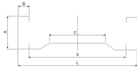
M型檩条规格 Size of-shape purline
