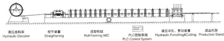
C型钢工艺流程图 C Purlin Machine Flow Chart
