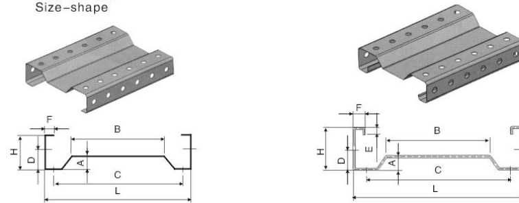
M型檩条机规格 Size-shape
