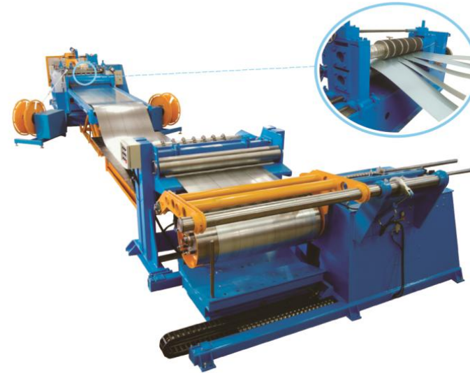
3.0毫米厚板纵剪线 3.0MM THICK HEAVY DUTY SLITTING LINE
