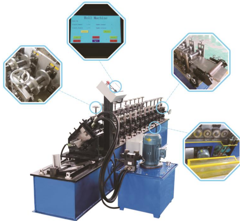
50/75/100龙骨成型机 50/75/100 CU STUD&TRACK ROLL FORMING MACHINE
